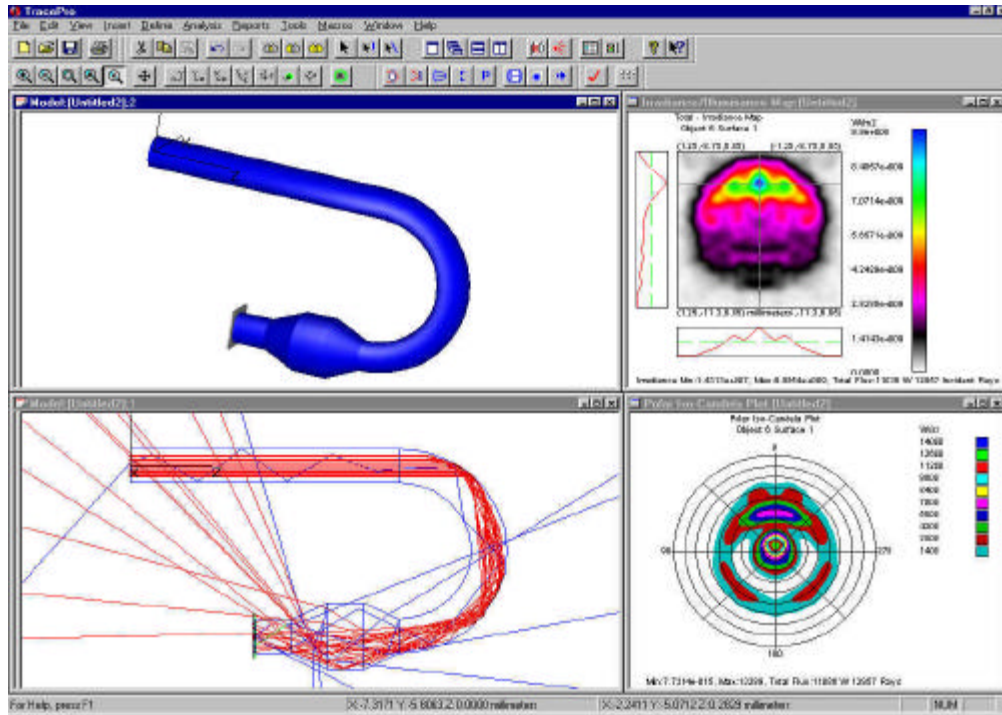
Figure 3 – Rendered light pipe with rays traced, irradiance and iso-candela maps shown
