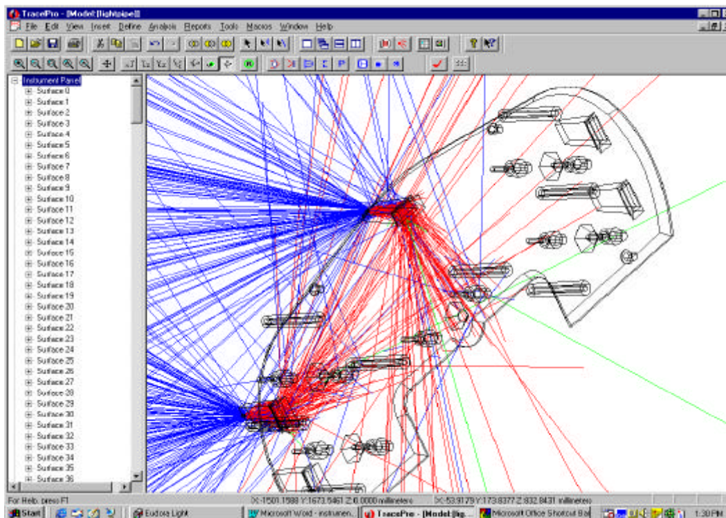
Figure 7 – Two LEDs emitting into the polycarbonate instrument panel
