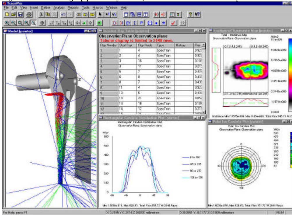
Figure 4 – Rendered speedometer pointer with rays traced, rectangular and regular iso-candela plots and irradiance map. Also a tabular ray history of the first 12 rays that reached the observation plane
