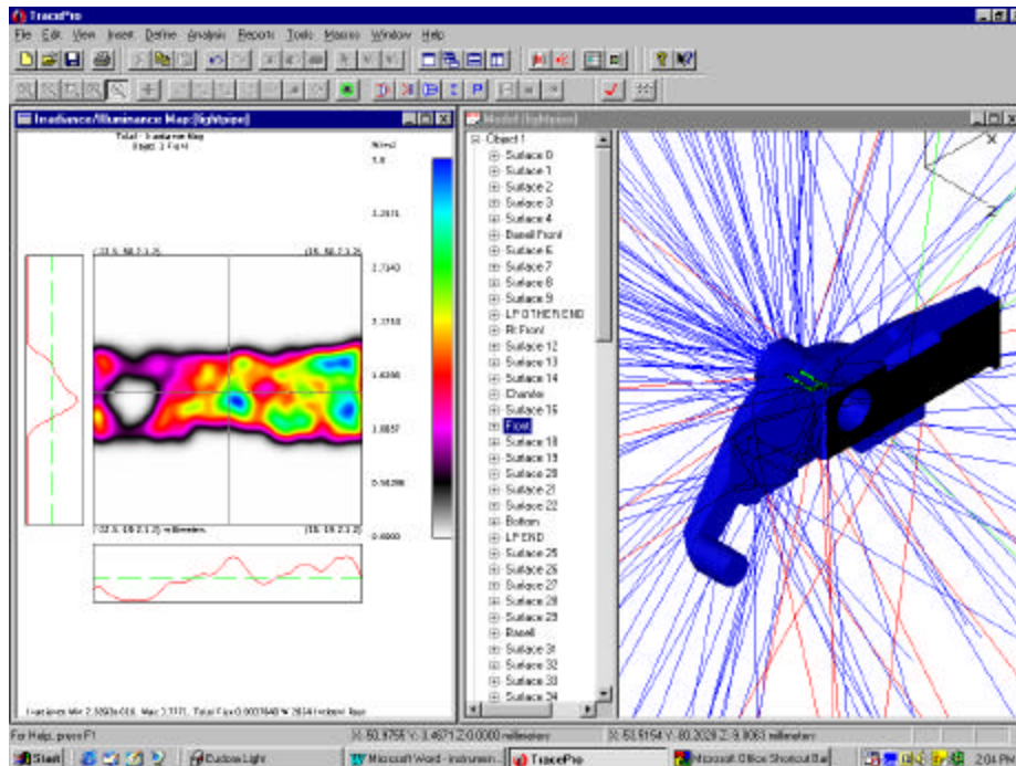
Figure 8 – Lightpipe for illuminating the air conditioning controls in a car. The irradiance map at left shows the Output of the lightpipe on it front right face in false color which is highlighted in black in the right plot.
