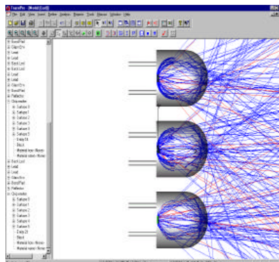
Figure 2 – Silhouette view of 3 common LEDs Shown emitting
